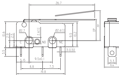
KW12-D628-□□
