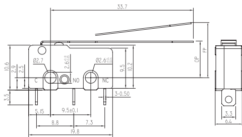
KW12-22GC-□□
